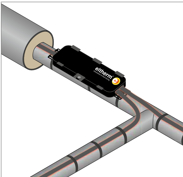
T型支路应用举例 / Application example Tee-splice
