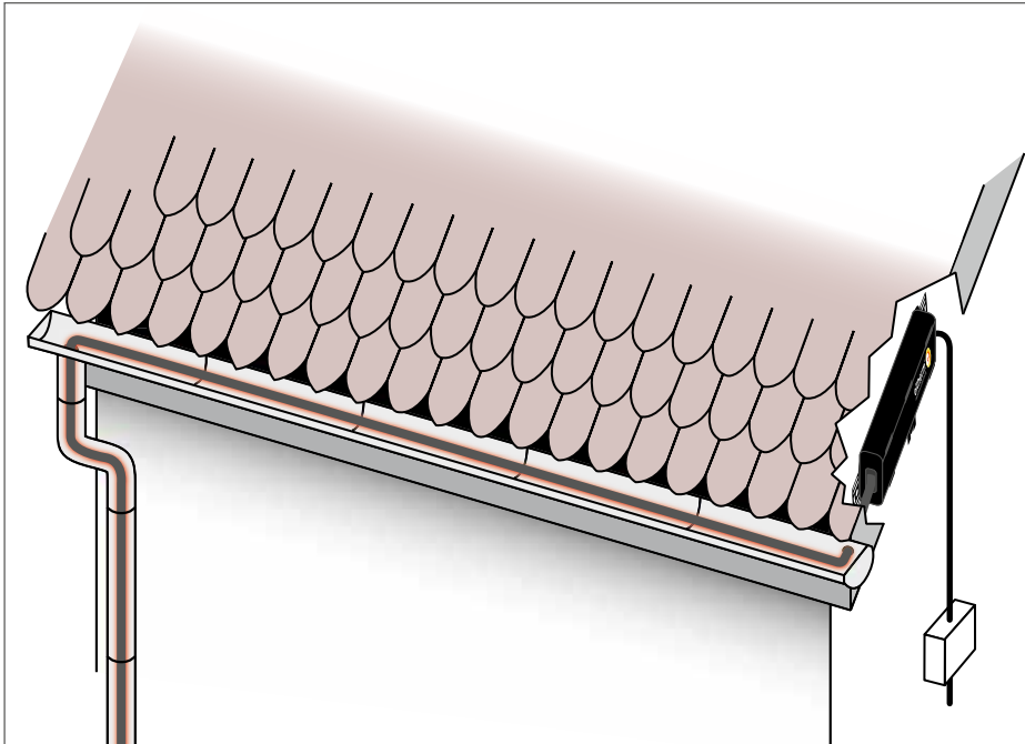
屋檐应用举例 / Application example gutter heating
